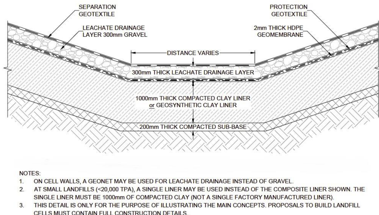
Figure 1 General solid waste landfill liner system
