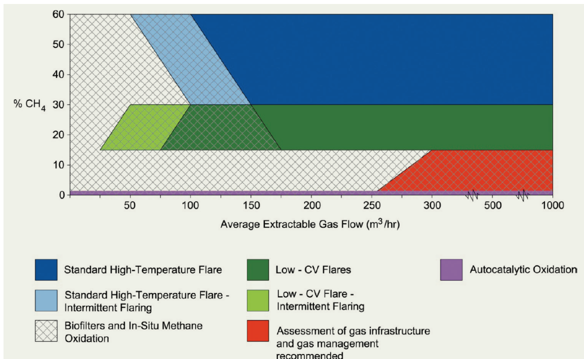
Figure 14 Technologies for landfill gas treatment based on percent methane composition and gas flow rate (Source: EPA Ireland 2011)
