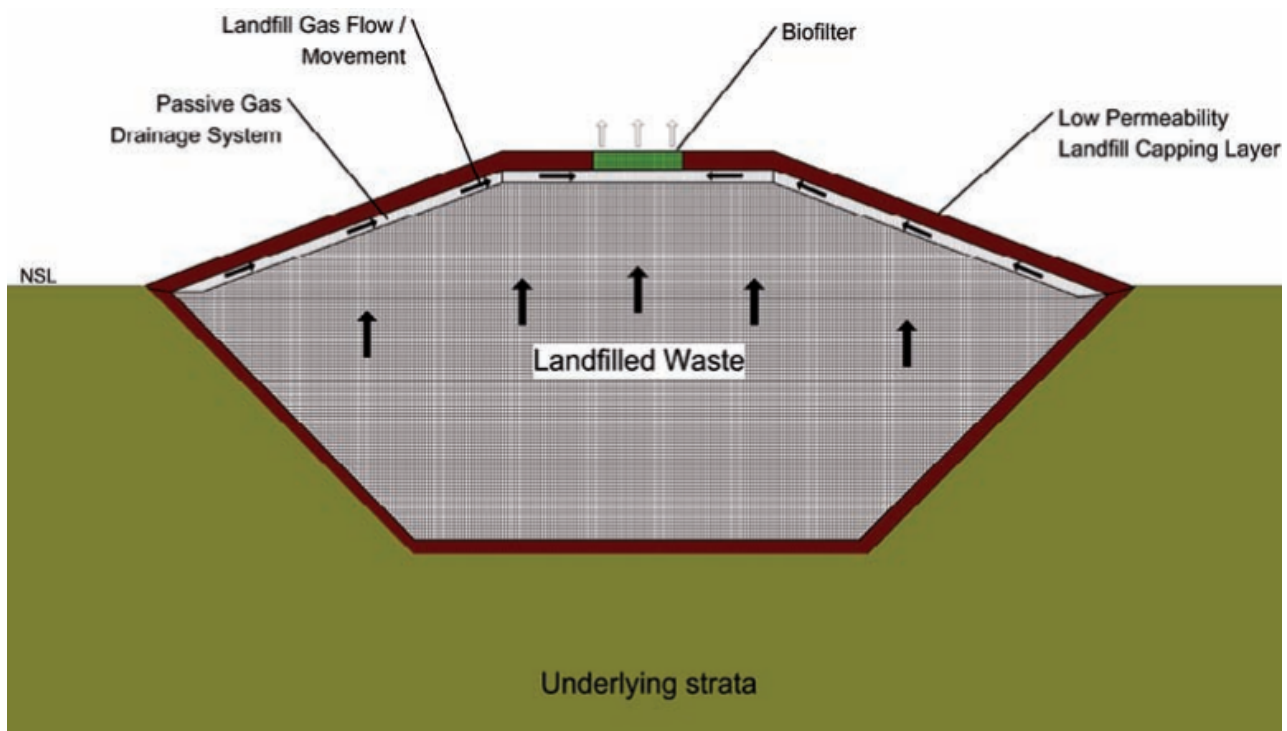
Figure 15 Concept drawing of a passive landfill gas drainage and biofiltration system
