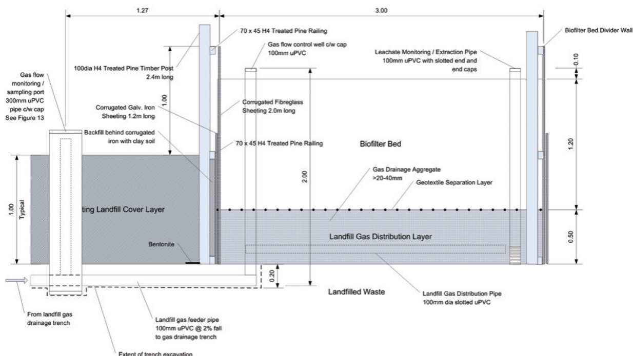
Figure 16 Typical section of a biofilter bed
